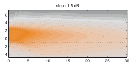
Step Array SA300S+ vertical directivity: sound level for the speech octaves (500Hz-1kHz-2kHz) in the vertical median plane.
