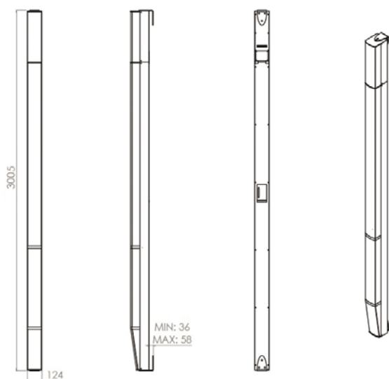
Front views
