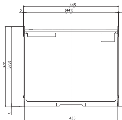
Top views
