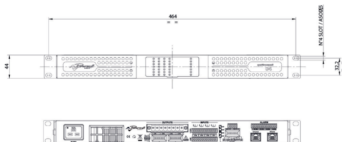
Front views
